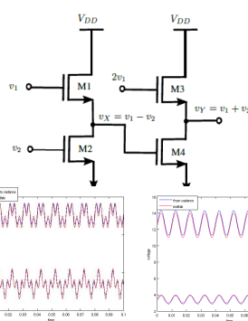
Adder subtractor
