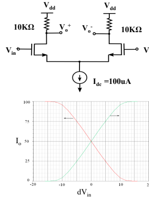
Diff amp
