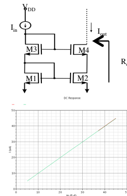
Cascode CM
